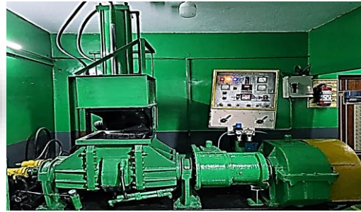
KNEADER MIXING
