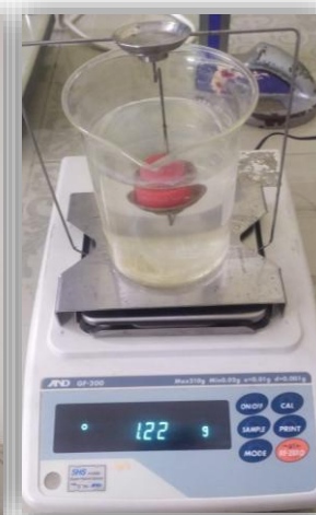
Density Tester
